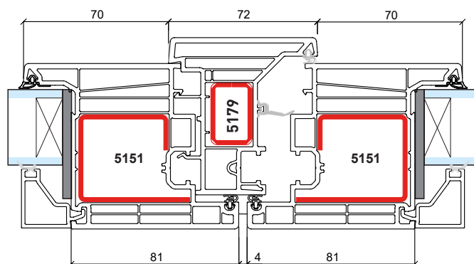
SECTION B
