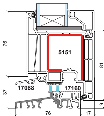
SECTION B
